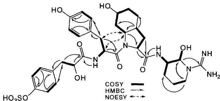
Fig.2 COSY, HMBC and NOESY correlations of Aeruginosin 102-A
