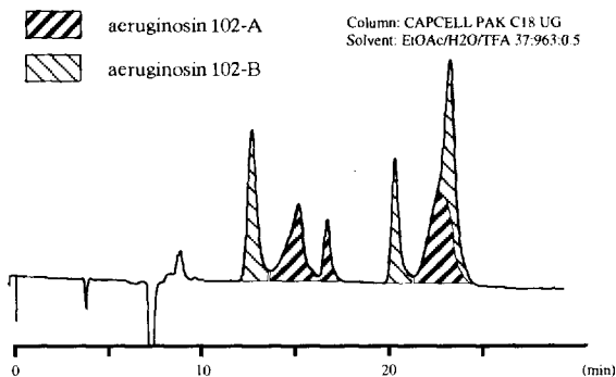
Fig. 1 HPLC chromatogram of aeruginosins 102-A, B
