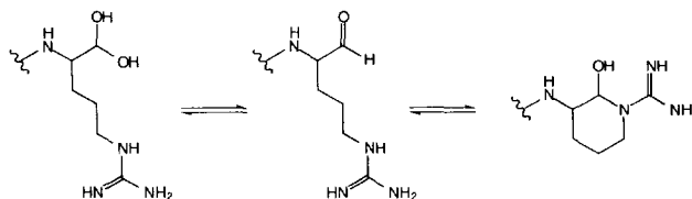
Fig. 4 Tautomerization of Argal
