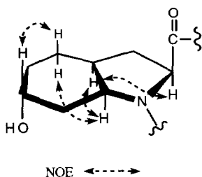
Fig. 3 Relative stereochemistry of Choi
